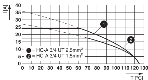
Derating diagram: Series HC-A 3-E..S / HC-A 4-E..S
