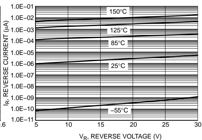
Figure 2. Reverse Leakage
