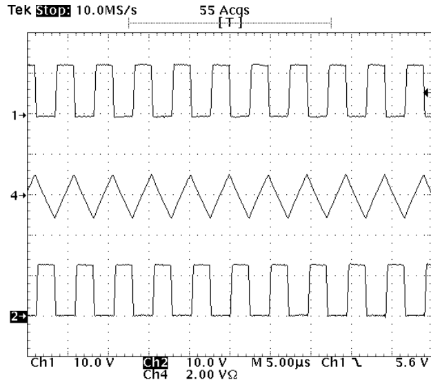
Figure 1 - Normal condition at no load. Ch1: HDrv Ch2: LDrv Ch4: Inductor Current
