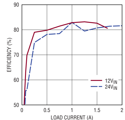
Efficiency vs Load Current, V_{OUT} = -18\text{V} , BIAS Tied to LTM8003 GND
