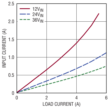
Input vs Load Current V_{OUT} = -3.3\text{V} , BIAS Tied to LTM8003 GND
