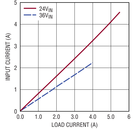
Input vs Load Current V_{OUT} = 18\text{V} , BIAS = 5V
