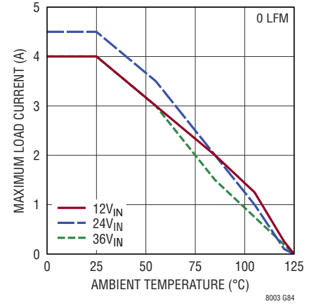
Derating, I-Grade, V_{OUT} = -15\text{V} , BIAS Tied to LTM8003 GND, DC2416A Demo Board
