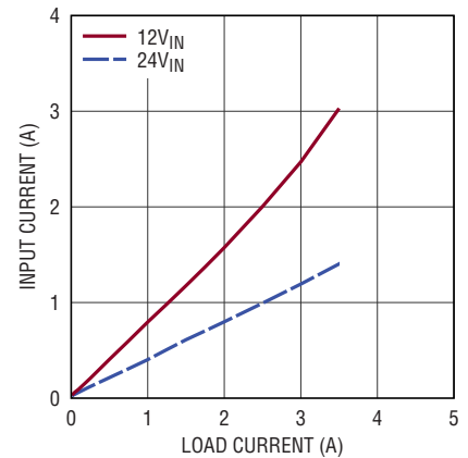
Input vs Load Current V_{OUT} = -8\text{V} , BIAS Tied to LTM8003 GND
