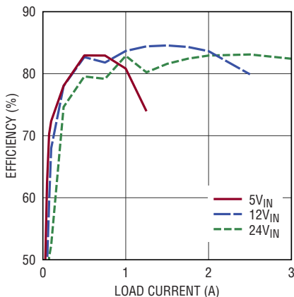
Efficiency vs Load Current, V_{OUT} = -12\text{V} , BIAS Tied to LTM8003 GND
