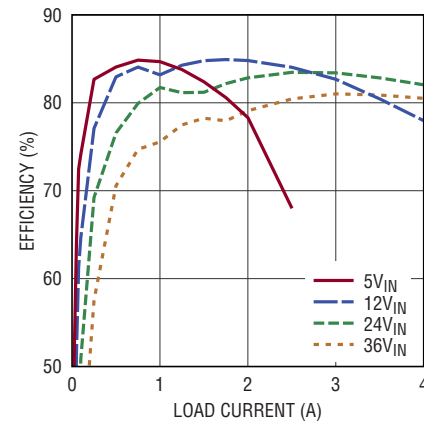
Efficiency vs Load Current, V_{OUT} = -5\text{V} , BIAS Tied to LTM8003 GND
