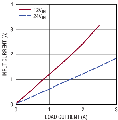
Input vs Load Current V_{OUT} = -12\text{V} , BIAS Tied to LTM8003 GND
