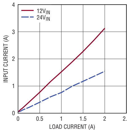
Input vs Load Current V_{OUT} = -15\text{V} , BIAS Tied to LTM8003 GND
