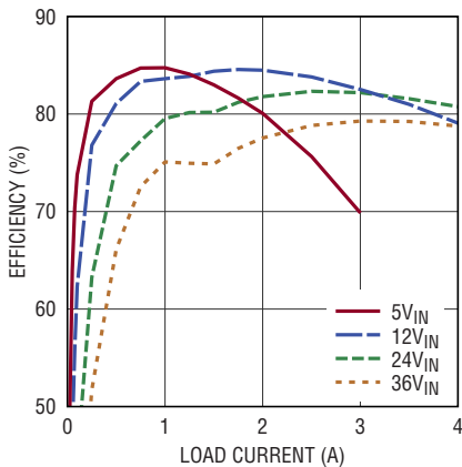
Efficiency vs Load Current, V_{OUT} = -3.3\text{V} , BIAS Tied to LTM8003 GND
