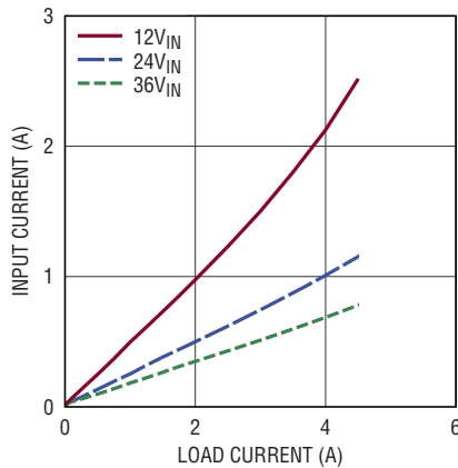
Input vs Load Current V_{OUT} = -5\text{V} , BIAS Tied to LTM8003 GND
