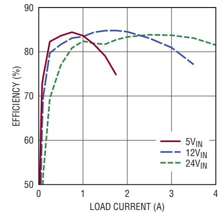
Efficiency vs Load Current, V_{OUT} = -8\text{V} , BIAS Tied to LTM8003 GND
