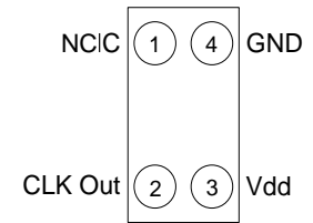
Figure 1. Pin Assignment
