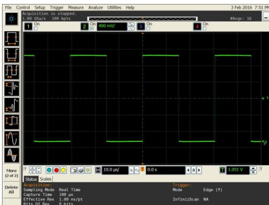
Figure 7. LVCMOS Output Sing
