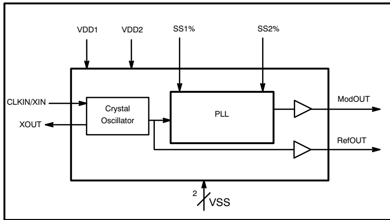
Figure 1. Block Diagram
