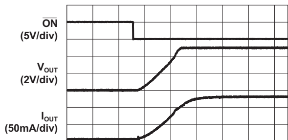
Time (40μs/div)
