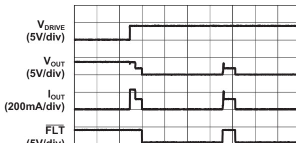
Time (10ms/div)
