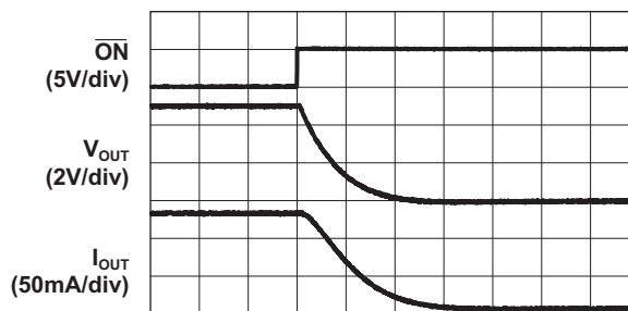
Time (40μs/div)
