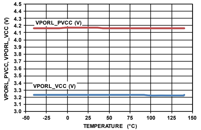
FIGURE 44. PVCC/VCC POR FALLING THRESHOLD vs TEMPERATURE
