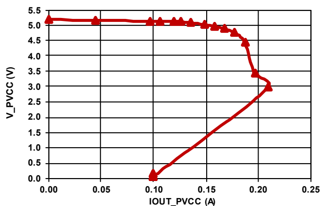
FIGURE 62. INTERNAL LDO OUTPUT VOLTAGE vs LOAD
