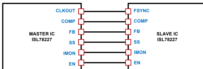
FIGURE 54. CONFIGURATIONS FOR DUAL IC 4-PHASE OPERATION
