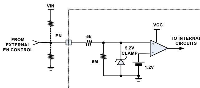
FIGURE 59. ENABLE BLOCK
