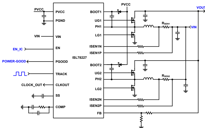
FIGURE 1. SIMPLIFIED APPLICATION SCHEMATIC, 2-PHASE SYNCHRONOUS BOOST
