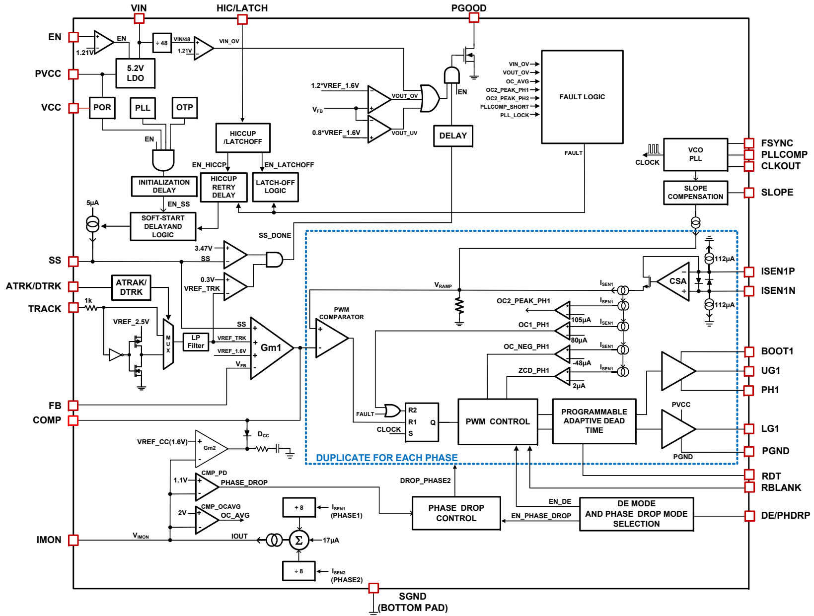
FIGURE 3. BLOCK DIAGRAM
