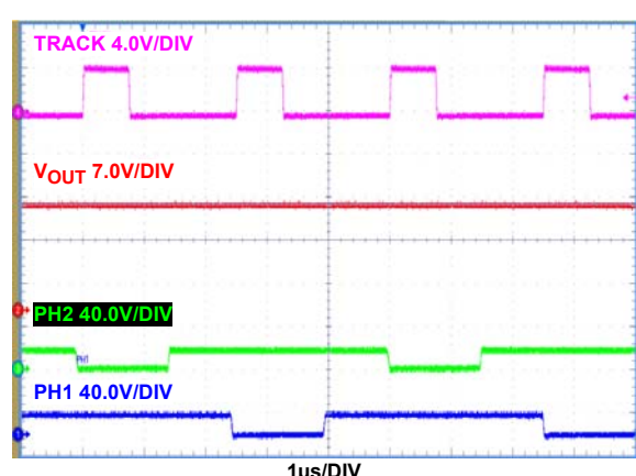
FIGURE 28. DIGITAL TRACKING (TRACKING SIGNAL, FREQUENCY = 400kHz, D = 0.3), V_{OUT} = 17V
