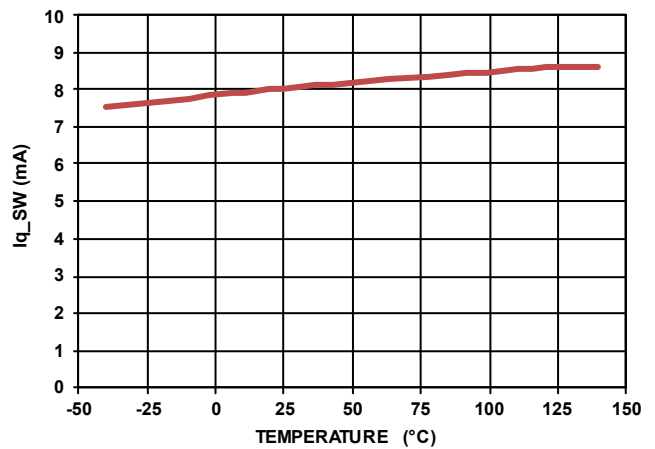
FIGURE 34. IC OPERATIONAL QUIESCENT CURRENT vs TEMPERATURE, IC SWITCHING, NO LOAD ON LGX AND UGX
