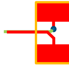
FIGURE 68. RECOMMENDED LAYOUT PATTERN FOR CURRENT SENSE TRACES REGULATOR
