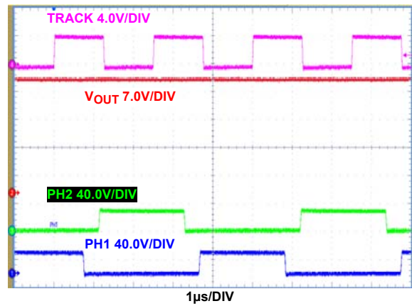
FIGURE 26. DIGITAL TRACKING (TRACKING SIGNAL, FREQUENCY = 400kHz, D = 0.5, V_{OUT} = 28.3V )
