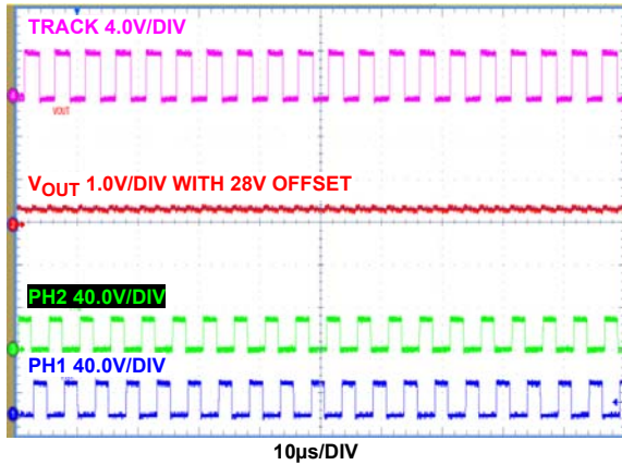
FIGURE 29. DIGITAL TRACKING, (TRACKING SIGNAL, FREQUENCY = 200kHz, D = 0.5), V_{OUT} = 28.3V
