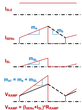
FIGURE 61. SLOPE COMPENSATION BLOCK DIAGRAM
