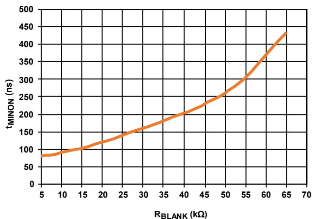
FIGURE 57. t_{MINON} vs RBLANK
