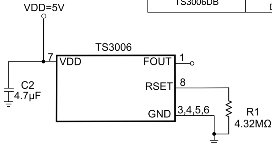
Figure 1. TS3006 Demo Board Circuit
