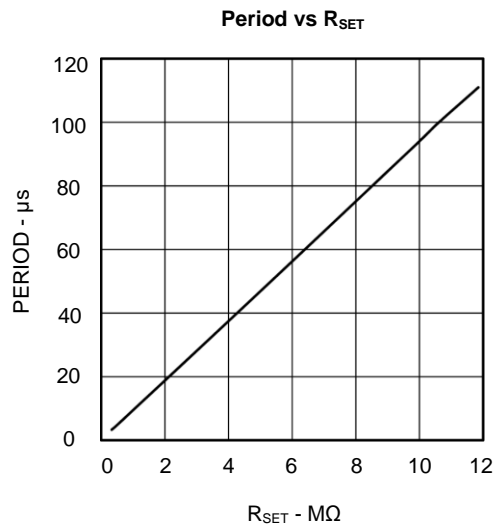
Figure 2. FOUT Period vs R_{SET}
