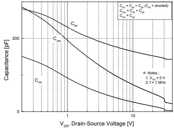
Fig.8 Capacitance Characteristics
