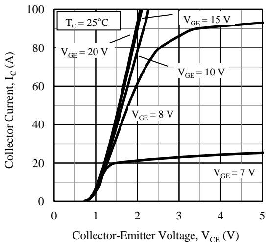
Figure 5. Output Characteristics (T C = 25 °C)
