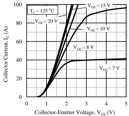
Figure 6. Output Characteristics (T C = 125 °C)
