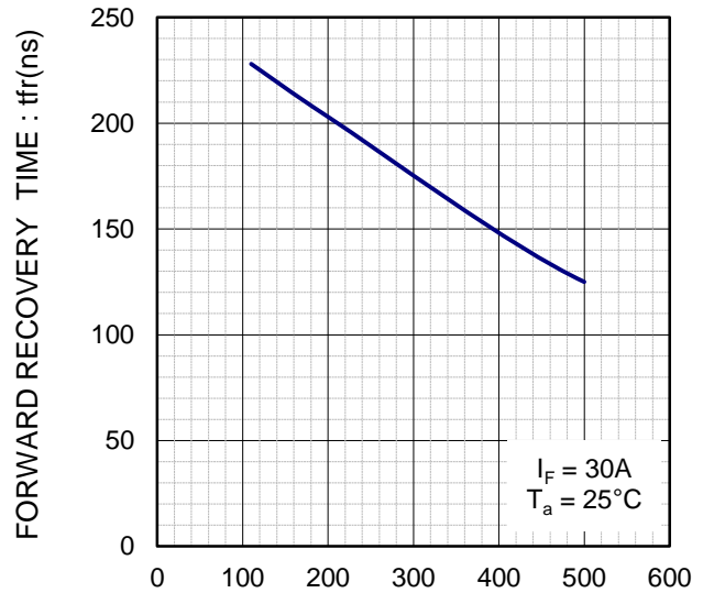
di/dt-t fr CHARACTERISTICS
