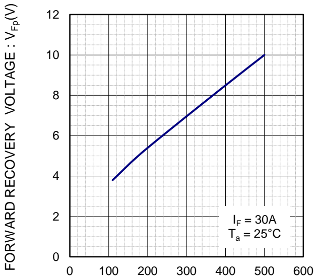
di/dt-V Fp CHARACTERISTICS
