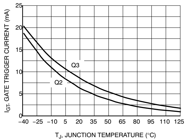
Figure 2. Typical Gate Trigger Current
