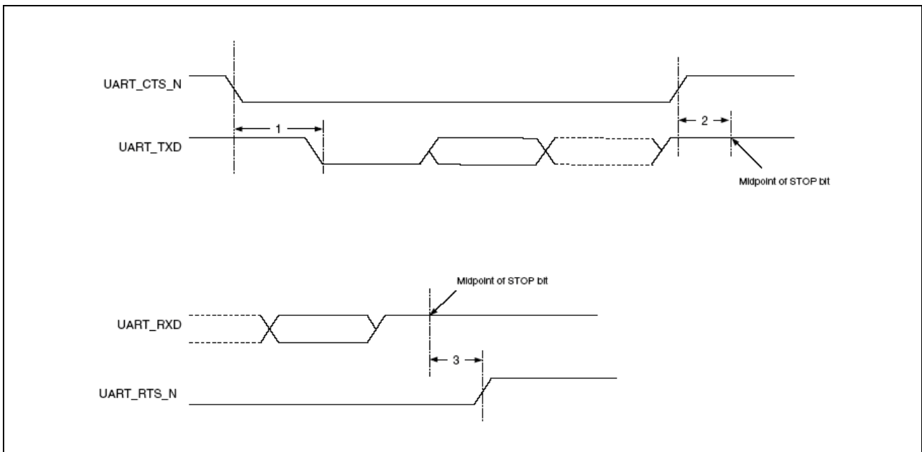
Figure 10: UART Timing
