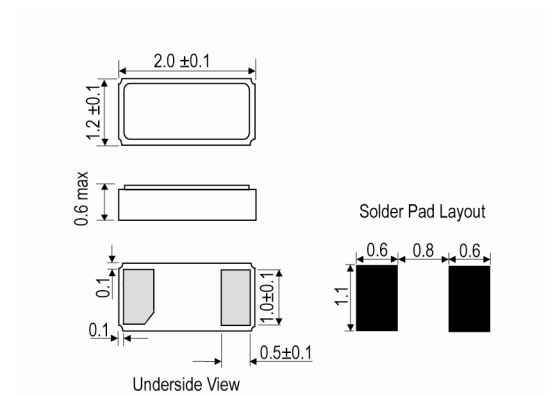
Outline (mm)
