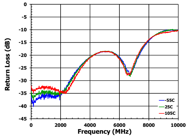
Figure 9. Evaluation Board Loss vs. Frequency
