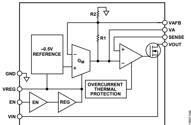
Figure 40. Fixed Output Voltage Internal Block Diagram
