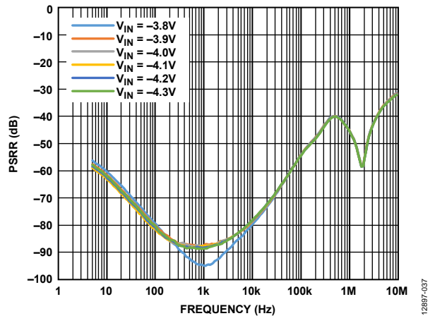
Figure 33. Power Supply Rejection Ratio (PSRR) vs. Frequency at Various Input Voltages, V_{OUT} = -3.3\text{ V} , I_{LOAD} = -300\text{ mA}
