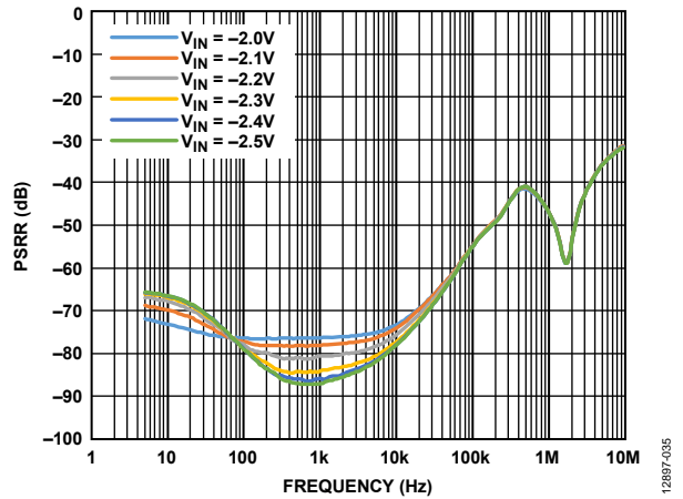
Figure 31. Power Supply Rejection Ratio (PSRR) vs. Frequency at Various Input Voltages, V_{OUT} = -1.2\text{ V} , I_{LOAD} = -300\text{ mA}
