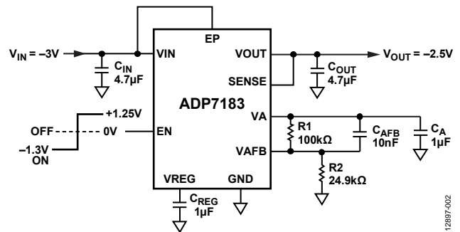
Figure 2. ADP7183 with Adjustable Output Voltage, V_{OUT} = -2.5 V
