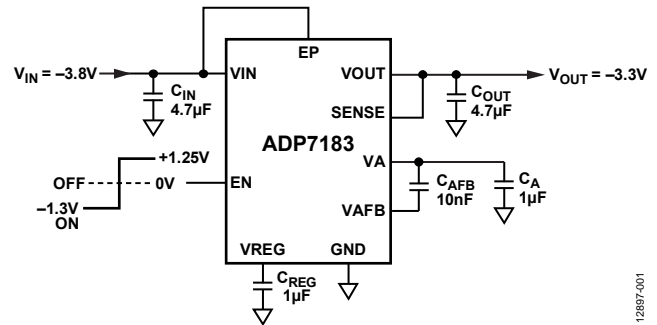
Figure 1. ADP7183 with Fixed Output Voltage, V_{OUT} = -3.3 V
