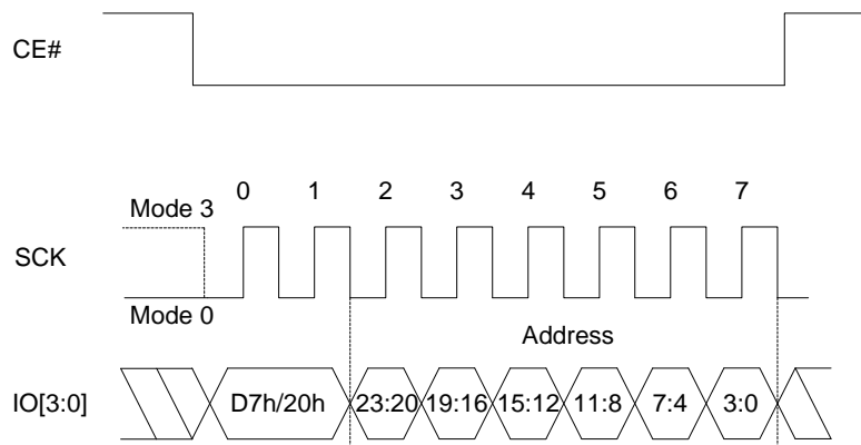
Figure 8.15 Sector Erase Sequence (QPI)
