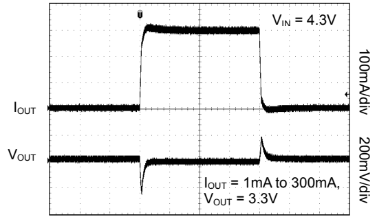
Time (100µs/div)
