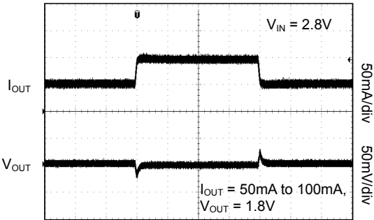
Time (100µs/div)
