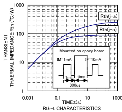
Rth-t CHARACTERISTICS
