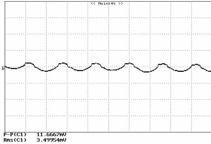
Figure 7: Output ripple & noise at 5Vin, 3.3V/3A out
