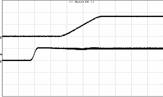
Figure 13: Turn on delay time at 5Vin, 3.3V/3A out
