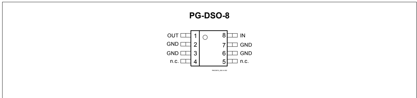
Figure 2 Pin Configuration
