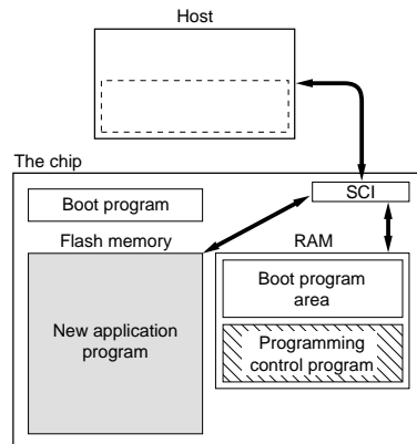
Figure 22.4 Boot Mode
