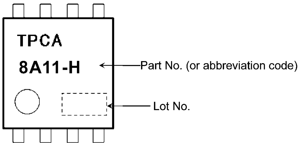
Fig. 7.1 Marking
