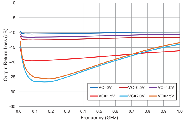
Output Return Loss versus Frequency RFSA3023, V_{DD}=3.3V , Temp=+25°C
