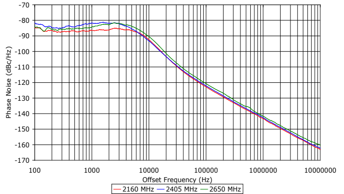
Phase Noise
