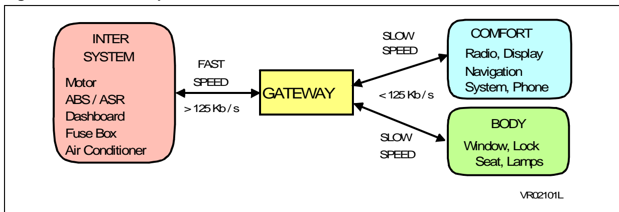
Figure 13. CAN Principle
