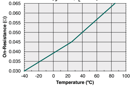
Typical On-Resistance vs. Temperature DC-Only Configuration ( I_F=0mA, I_L=1.5A )
