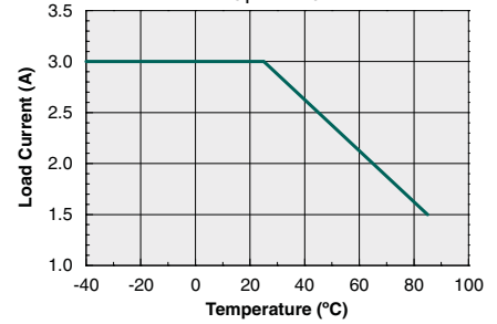
Maximum Load Current vs. Temperature DC-Only Configuration ( I_F=0mA )
