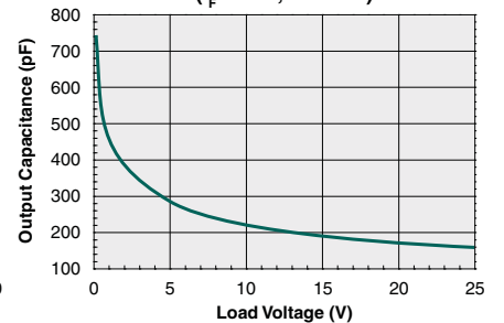
Output Capacitance vs. Load Voltage ( I_F=2mA, f=1MHz )
