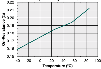
Typical On-Resistance vs. Temperature AC/DC Configuration ( I_F=0mA, I_L=750mA )
