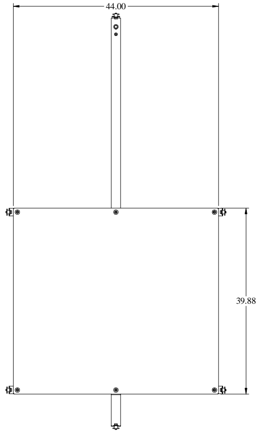
FRONT VIEW
