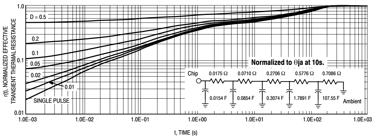
Figure 11. Thermal Response
