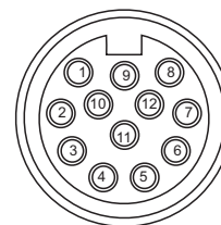
Male 12-pin Face view
