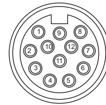
Female 12-pin Face view
