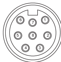
Female 8-pin Face view
