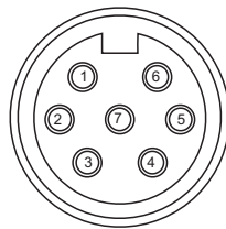
Female 7-pin Face view
