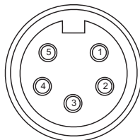
Female 5-pin - Face view
