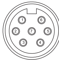
Male 7-pin Face view
