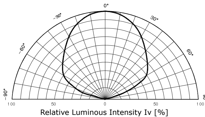
Fig. 5 Radiation Diagram
