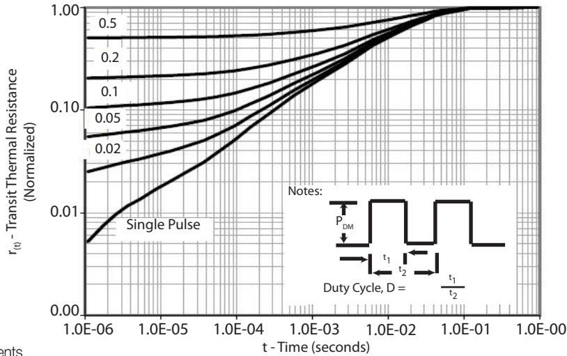
Transient Thermal Response - Junction to Case
