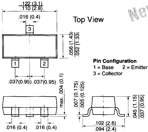
TO-236AB (SOT-23)
