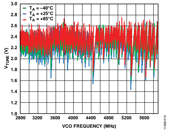
Figure 23. V_{TUNE} vs. VCO Frequency
