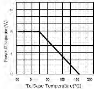
Fig.3 Power Derating
