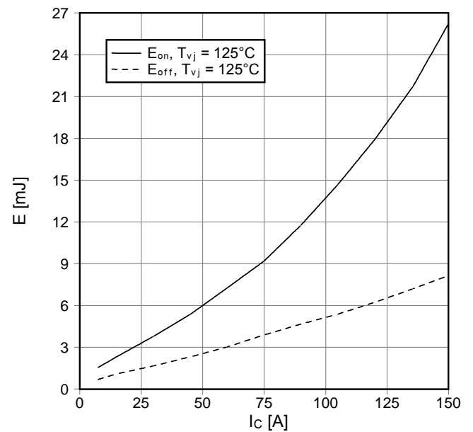
Schaltverluste IGBT-Wechselr. (typisch) switching losses IGBT-inverter (typical) E_{on} = f(I_C) , E_{off} = f(I_C) V_{GE} = \pm 15\text{ V} , R_{Gon} = 7,5\ \Omega , R_{Goff} = 7,5\ \Omega , V_{CE} = 600\text{ V}
