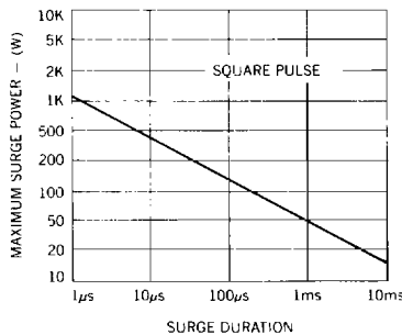
Maximum Surge Power vs Surge Duration
