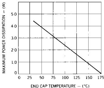
Power Dissipation vs End Cap Temperature Derating Curve
