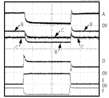
SYSTEM LOAD TRANSIENT
