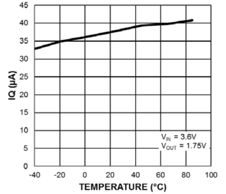
Quiscent Current vs. Temperature
