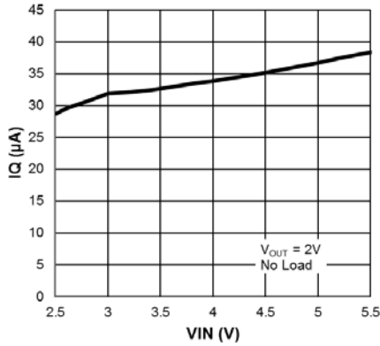
Quiscent Current vs. Input Voltage
