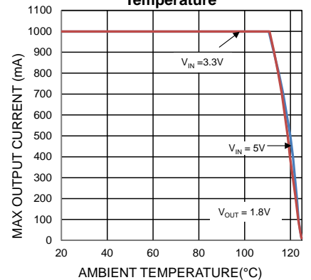
Max. Output Current vs. Temperature
