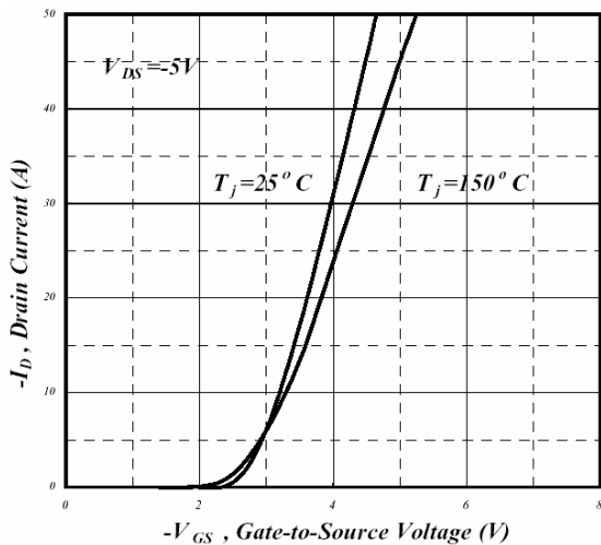
Fig 11. Transfer Characteristics
