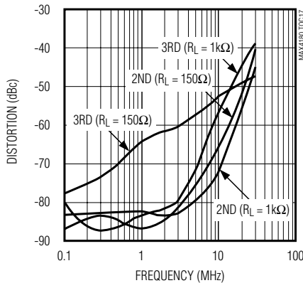
MAX4180 HARMONIC DISTORTION vs. FREQUENCY (SINGLE SUPPLY)
