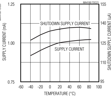
SUPPLY CURRENT (OPERATING & SHUTDOWN) vs. TEMPERATURE
