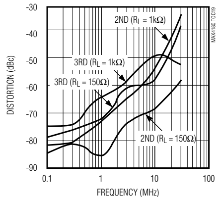
MAX4181 HARMONIC DISTORTION vs. FREQUENCY (SINGLE SUPPLY)
