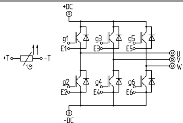
pinout, dimensions
