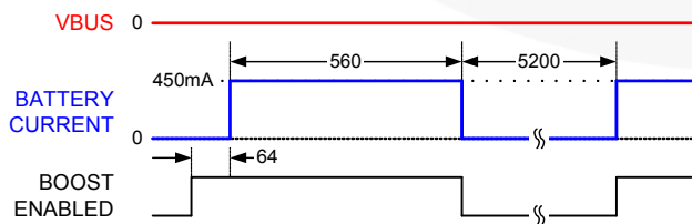
Figure 44. Boost Response Attempting to Start into VBUS Short Circuit (Times in µs)
