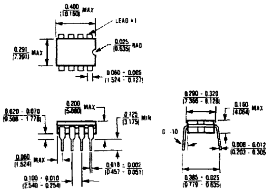
8 Lead Cerdip (JA) \theta_{JA} = 125^{\circ}\text{C/W} \theta_{JC} = 55^{\circ}\text{C/W}
