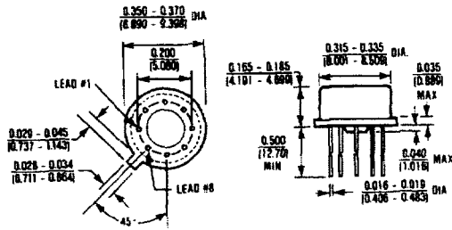
8 Lead TO-99 (TV) \theta_{JA} = 150^{\circ}\text{C/W} \theta_{JC} = 45^{\circ}\text{C/W}
