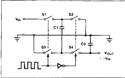
Figure 2. Idealized Negative Voltage Converter
