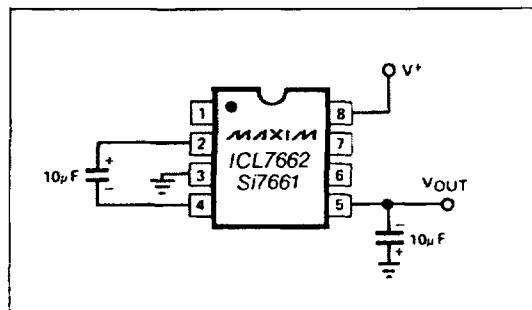
Figure 6. Negative Voltage Converter
