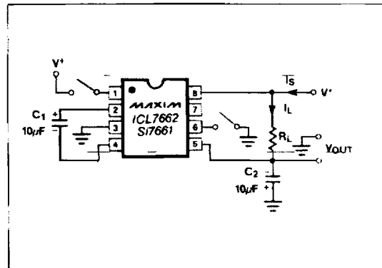
Figure 1. ICL7662/SI7661 Test Circuit
