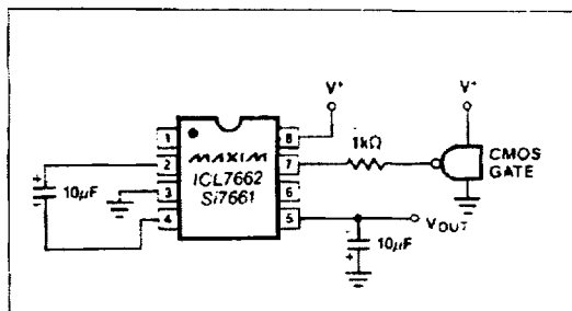
Figure 4. External Clocking
