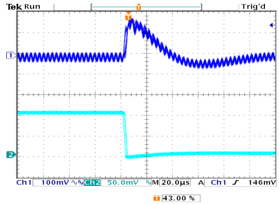
Figure 22: Typical transient response to step load change at 5A/\mu s from 100% to 50% of I_o , max at 12V_{in} , 5.0V out ( C_{out} = 1\mu F + 100\mu F ceramic, 470\mu F poscap).
