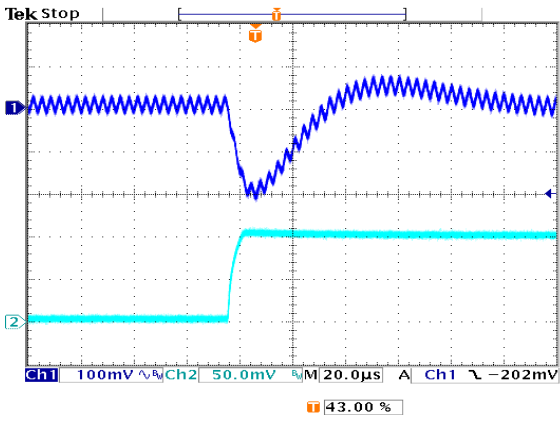
Figure 21: Typical transient response to step load change at 5A/\mu s from 50% to 100% of I_o , max at 12V_{in} , 5.0V out ( C_{out} = 1\mu F + 100\mu F ceramic, 470\mu F poscap).
