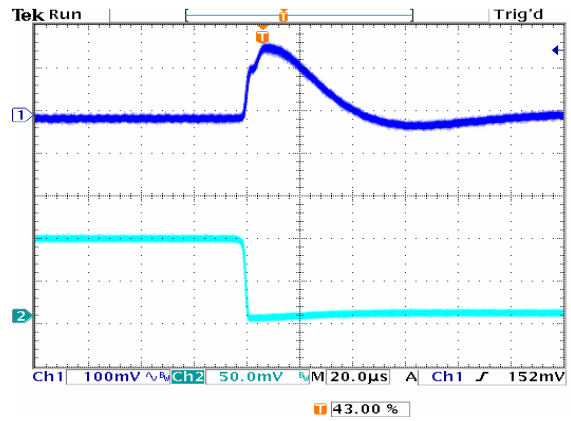
Figure 16: Typical transient response to step load change at 5A/ \mu S from 100% to 50% of Io, max at 12Vin, 0.75V out (Cout = 1 \mu F+ 100 \mu F ceramic, 470 \mu F poscap).
