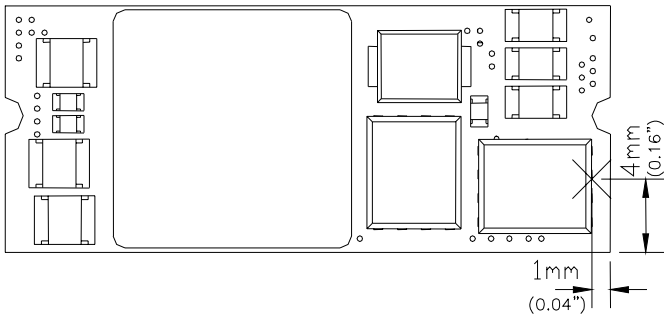
Figure 39: Temperature measurement location * The allowed maximum hot spot temperature is defined at 125
