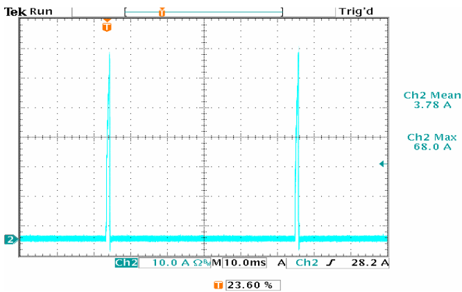
Figure 23: Output short circuit current 12V_{in} , 0.75V_{out} ( 10A/div )
