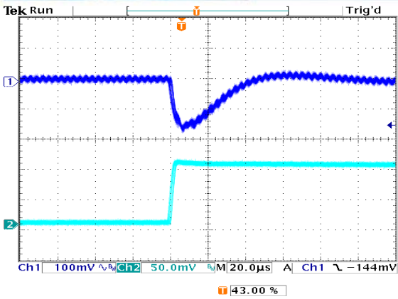
Figure 19: Typical transient response to step load change at 5A/\mu s from 50% to 100% of I_o , max at 12V_{in} , 2.5V out ( C_{out} = 1\mu F + 100\mu F ceramic, 470\mu F poscap).
