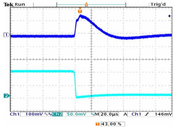
Figure 18: Typical transient response to step load change at 5A/ \mu S from 100% to 50% of Io, max at 12Vin, 1.2V out (Cout = 1 \mu F+ 100 \mu F ceramic, 470 \mu F poscap).
