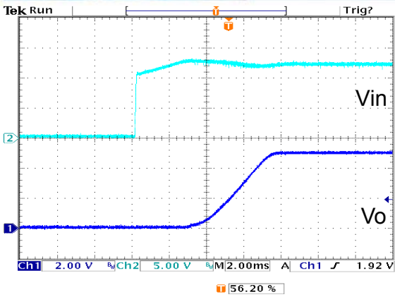
Figure 13: Turn on at 12Vin, with external capacitors (Co= 5000 \mu F), 5.0V/20A out
