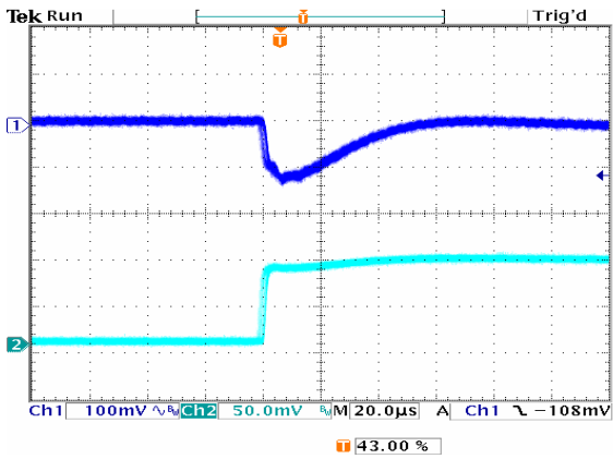
Figure 15: Typical transient response to step load change at 5A/ \mu S from 50% to 100% of Io, max at 12Vin, 0.75V out (Cout = 1 \mu F+ 100 \mu F ceramic, 470 \mu F poscap).
