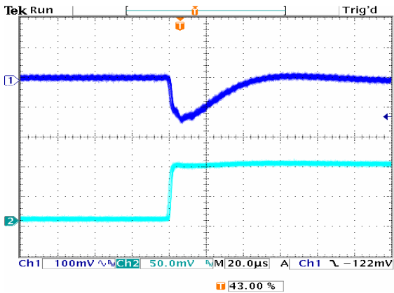
Figure 17: Typical transient response to step load change at 5A/ \mu S from 50% to 100% of Io, max at 12Vin, 1.2V out (Cout = 1 \mu F+ 100 \mu F ceramic, 470 \mu F poscap).
