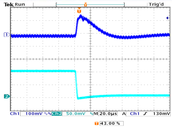
Figure 20: Typical transient response to step load change at 5A/\mu s from 100% to 50% of I_o , max at 12V_{in} , 2.5V out ( C_{out} = 1\mu F + 100\mu F ceramic, 470\mu F poscap).
