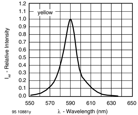
Figure 13. Relative Intensity vs. Wavelength
