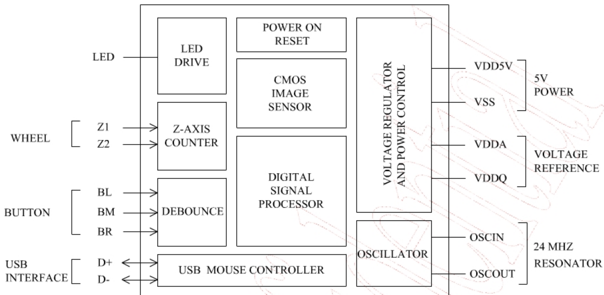
Figure 3. Block Diagram
