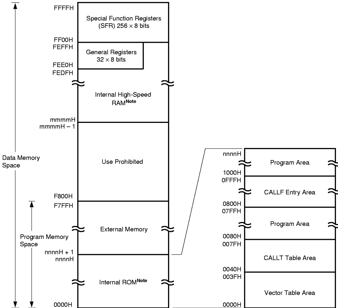
Figure 4-1. Memory Map
