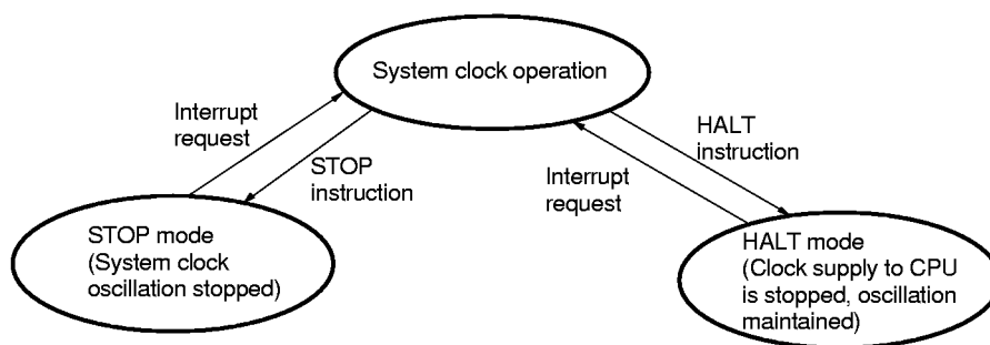
Figure 8-1. Standby Function
