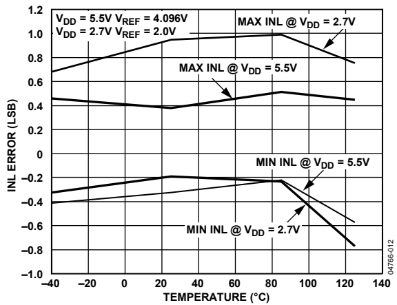
Figure 6. INL Error vs. Temperature
